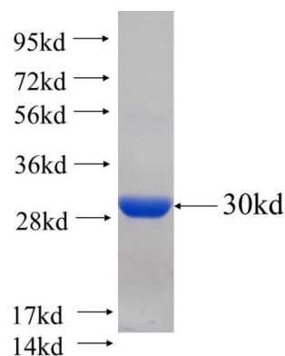
Recombinant Arabidopsis thaliana MOBP2 SDS-PAGE
