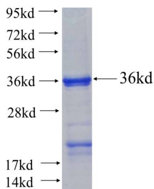
Recombinant human SURF2(Full length) SDS-PAGE
