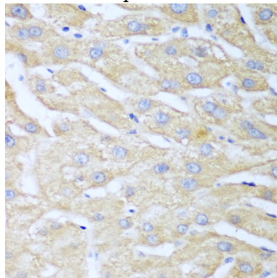
Immunohistochemistry - NUDT15 Polyclonal Antibody
