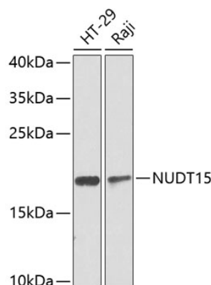
Western blot - NUDT15 Polyclonal Antibody
