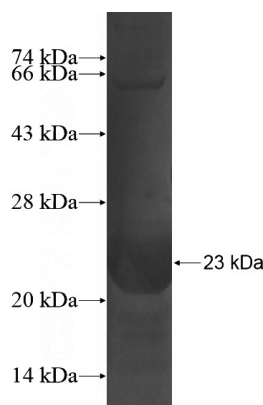
Recombinant Human C14orf126 SDS-PAGE
