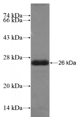
Recombinant Human APC SDS-PAGE
