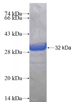
Recombinant Human Prohibitin SDS-PAGE
