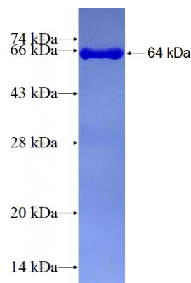
Recombinant Human OAS1 SDS-PAGE
