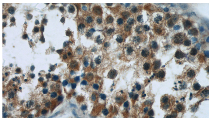
Immunohistochemistry of paraffin-embedded human testis tissue slide using Catalog No:111705(HSPH1 Antibody) at dilution of 1:50 (under 40x lens)
