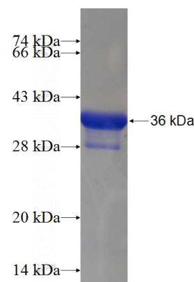
Recombinant Human LSM5 SDS-PAGE
