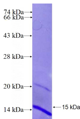
Recombinant Human BSCL2 SDS-PAGE
