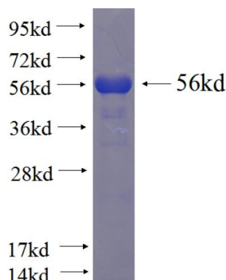
Recombinant human Tubulin-Alpha SDS-PAGE
