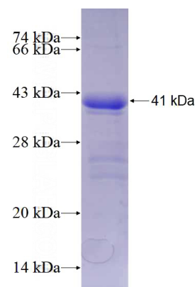
Recombinant Human FOXO3A SDS-PAGE
