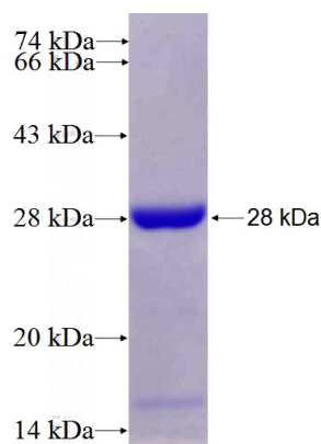
Recombinant Human TSG101 SDS-PAGE
