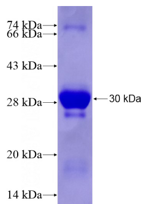
Recombinant Human PREB SDS-PAGE
