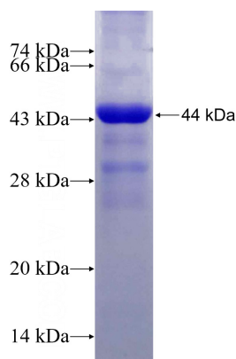
Recombinant Human RIN1 SDS-PAGE
