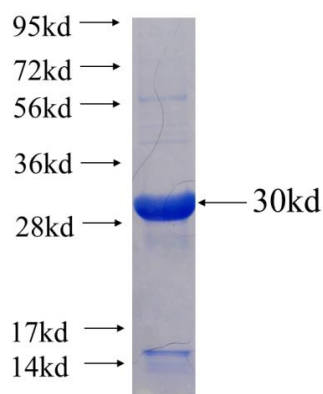
Recombinant Arabidopsis thaliana FAP3 SDS-PAGE
