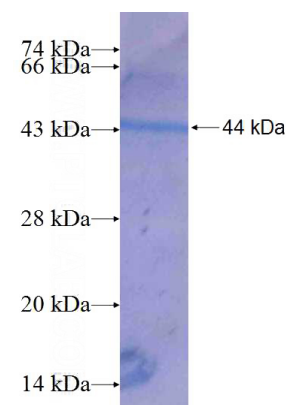
Recombinant Human NSUN3 SDS-PAGE
