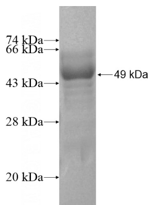
Recombinant Human RAB9B SDS-PAGE
