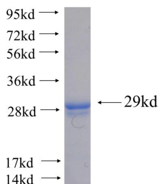
Recombinant human MED20(Full length) SDS-PAGE
