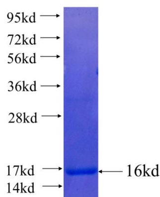
Recombinant human ACSL4 SDS-PAGE
