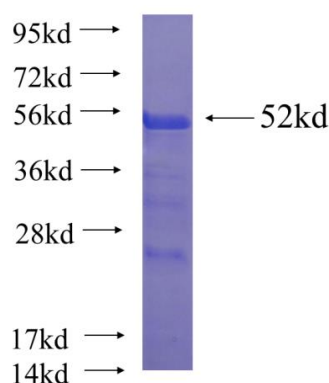
Recombinant human VWA5A SDS-PAGE
