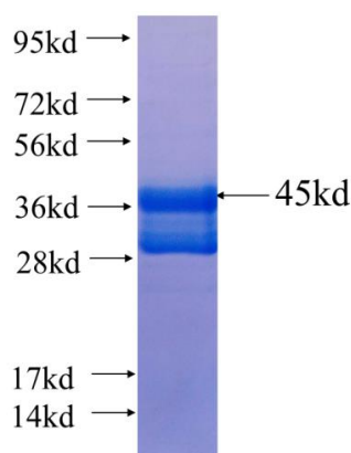
Recombinant human MBP(Full length) SDS-PAGE
