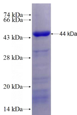
Recombinant Human STK38 SDS-PAGE
