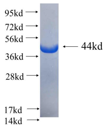
Recombinant Arabidopsis thaliana SHT SDS-PAGE
