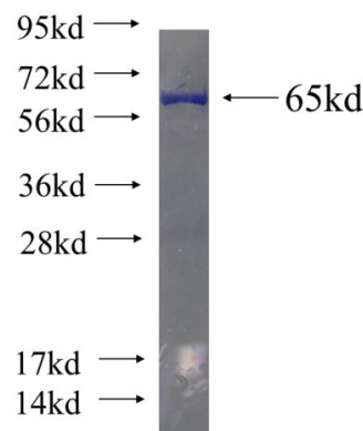
Recombinant Arabidopsis thaliana PTP1 SDS-PAGE
