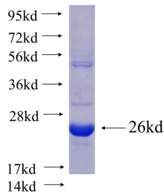
Recombinant Arabidopsis thaliana WHY2 SDS-PAGE
