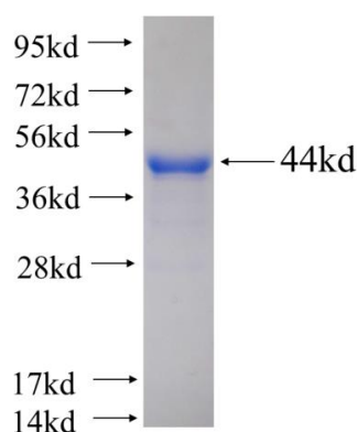
Recombinant Arabidopsis thaliana DHDPS2 SDS-PAGE
