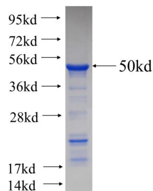
Recombinant Arabidopsis thaliana AtUVR8 SDS-PAGE
