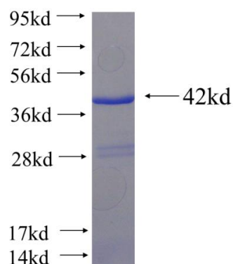
Recombinant Arabidopsis thaliana ACAM-2 SDS-PAGE
