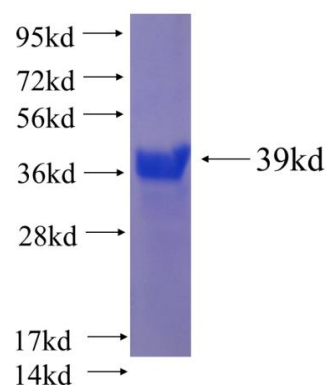
Recombinant Arabidopsis thaliana AtGRXS14 SDS-PAGE
