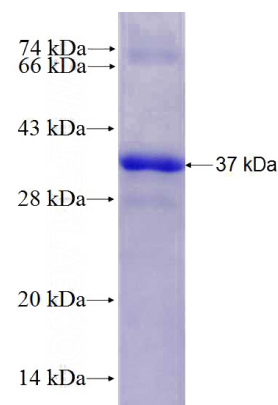
Recombinant Human CFTR SDS-PAGE
