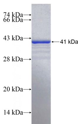
Recombinant Human NMDAR2A/GRIN2A SDS-PAGE
