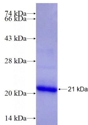
Recombinant Human ITGB3 SDS-PAGE
