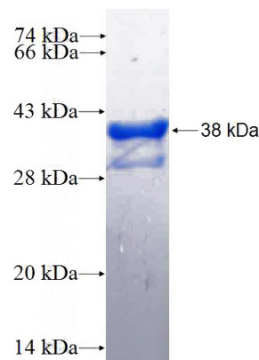
Recombinant Human TMC8 SDS-PAGE
