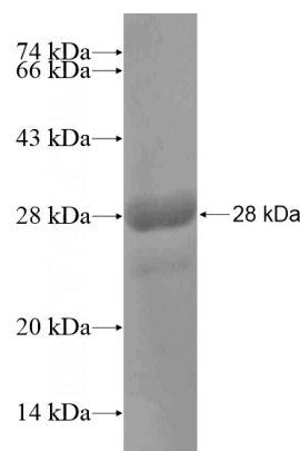
Recombinant Human FAM48A SDS-PAGE
