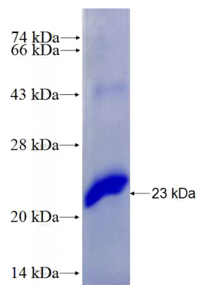
Recombinant Human CD18 SDS-PAGE
