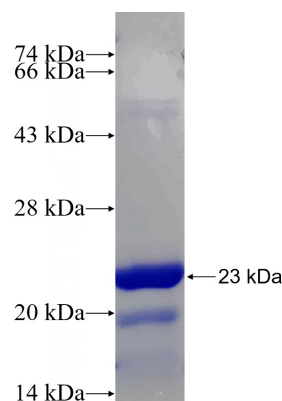
Recombinant Human DUB3 SDS-PAGE
