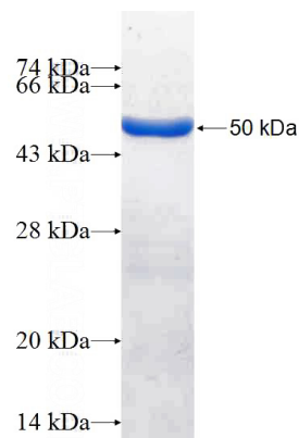
Recombinant Human Occludin SDS-PAGE
