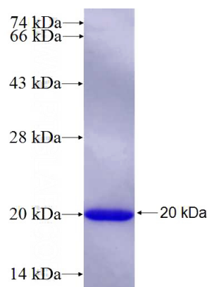
Recombinant Human DVL1 SDS-PAGE
