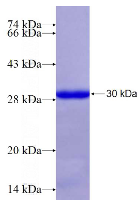
Recombinant Human ACOT2 SDS-PAGE
