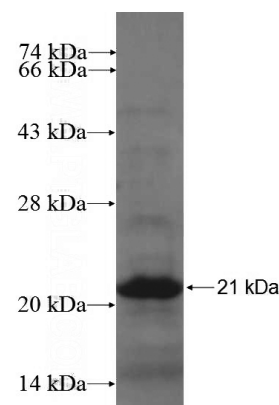
Recombinant Human HSD17B1 SDS-PAGE
