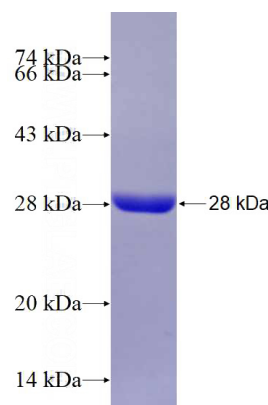
Recombinant Human CYP7A1 SDS-PAGE
