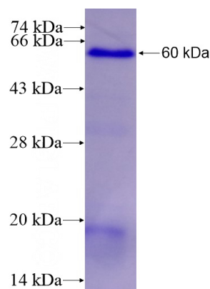
Recombinant Human NEK10 SDS-PAGE
