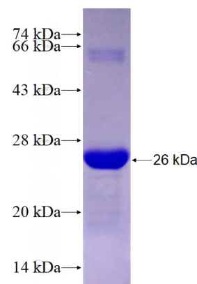
Recombinant Human SPATA17 SDS-PAGE
