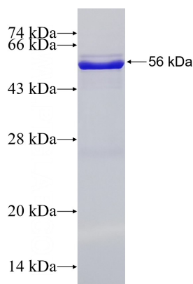
Recombinant Human P2RX4 SDS-PAGE
