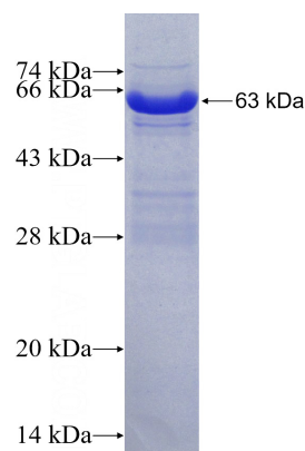
Recombinant Human NAGK SDS-PAGE
