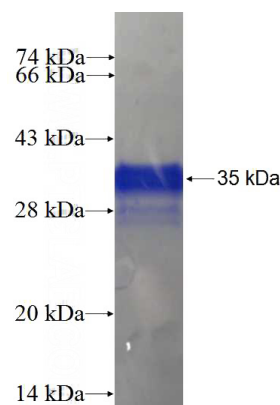
Recombinant Human AES SDS-PAGE
