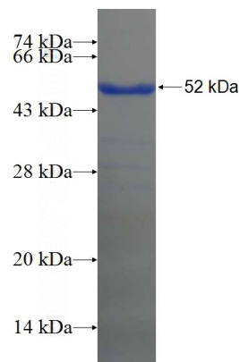
Recombinant Human MAST4 SDS-PAGE
