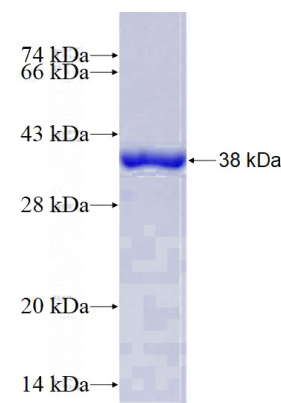
Recombinant Human TNNI3 SDS-PAGE
