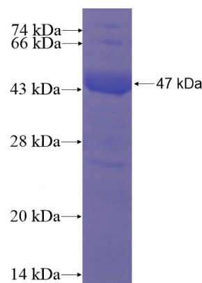
Recombinant Human ARL13B SDS-PAGE
